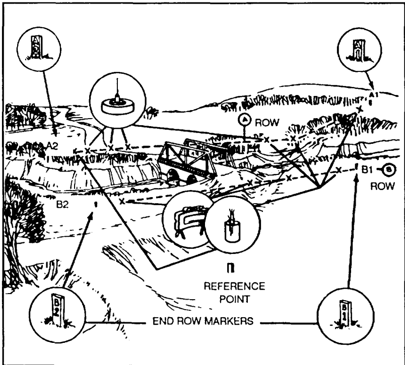
Figure 2-79. Leader visualizes hasty protective minefield.
